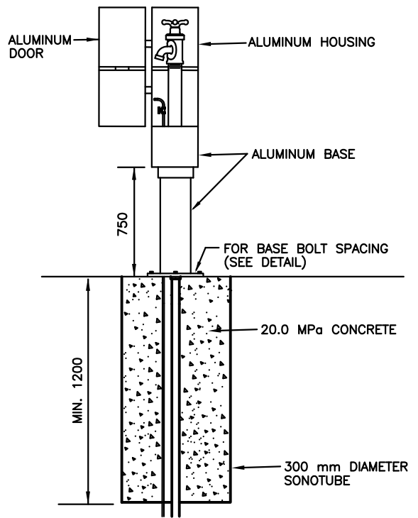
SAMPLING STATION ON PEDESTAL
