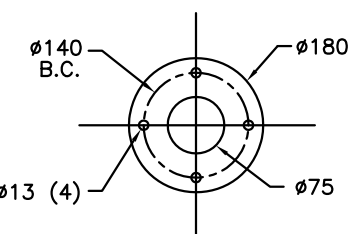
BASE BOLT SPACING DETAIL
