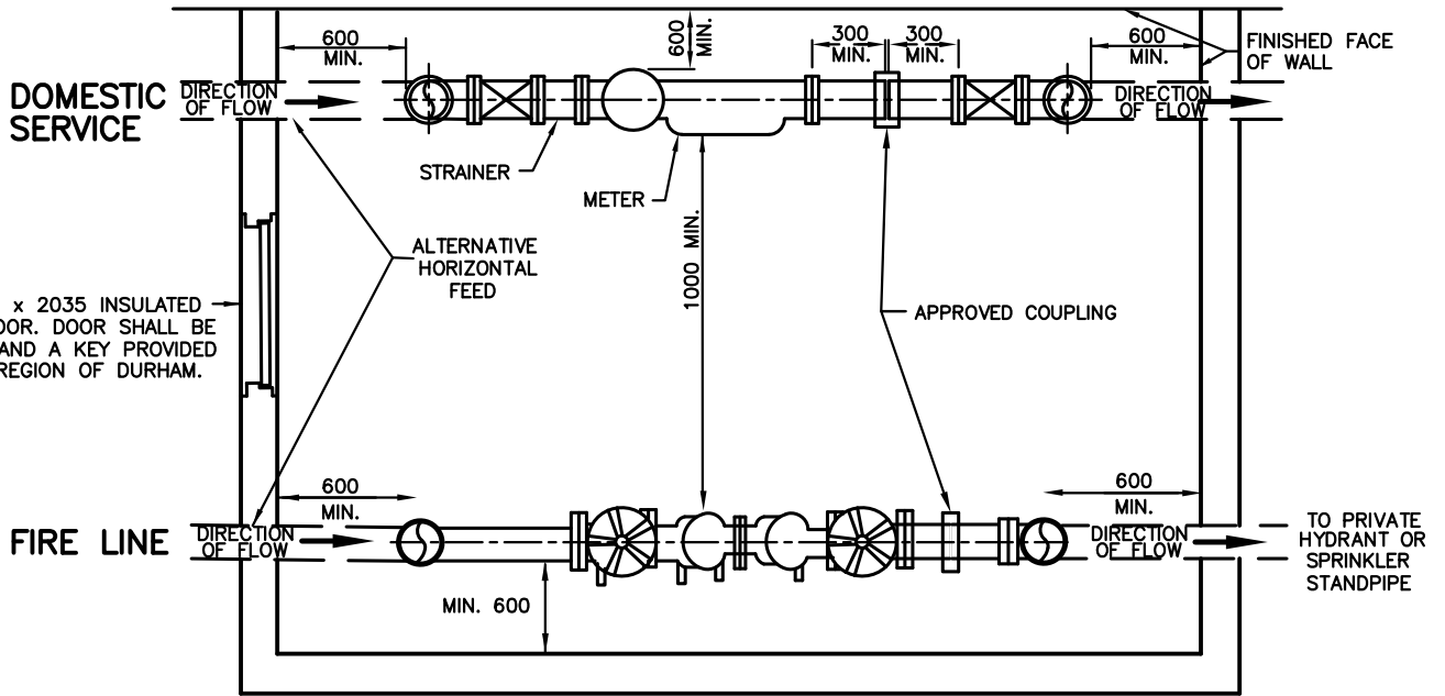
PLAN VIEW: TYPICAL VERTICAL DOMESTIC INSTALLATION / HORIZONTAL FIRE LINE INSTALLATION
