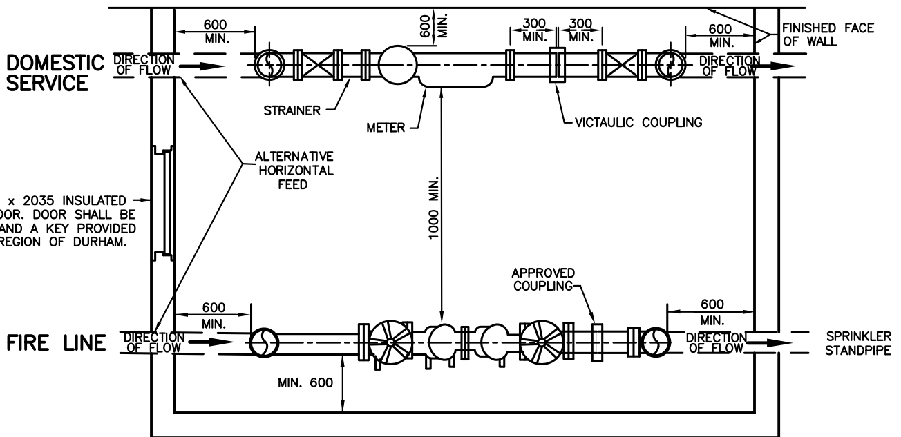
PLAN VIEW: TYPICAL DOMESTIC INSTALLATION / VERTICAL FIRE LINE INSTALLATION
